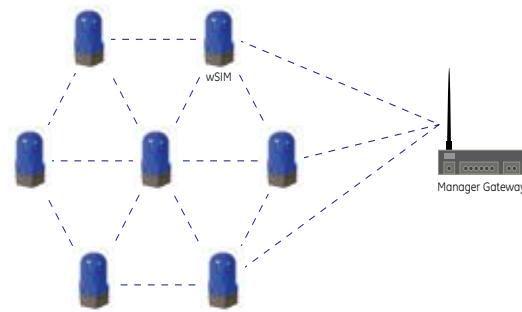
In a mesh network, each device is a peer that can talk to other peers, resulting in multiple signal transmission paths, higher reliability, and higher deployment flexibility.
